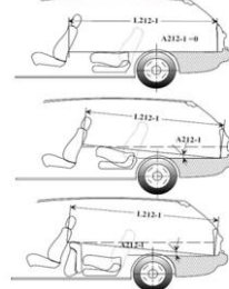
PART 3 – Description of the Package Drawing and Dimension List FIGURE 39-2: LUGGAGE FLOOR LENGTH – FIRST, L212-1, A212-1
