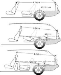
PART 3 – Description of the Package Drawing and Dimension List FIGURE 39-2: LUGGAGE FLOOR LENGTH – FIRST, L212-1, A212-1
