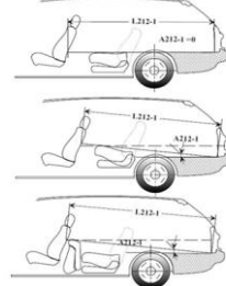
PART 3 – Description of the Package Drawing and Dimension List FIGURE 20-2: LUGGAGE FLOOR LENGTH – FIRST, L212-1, A212-1
